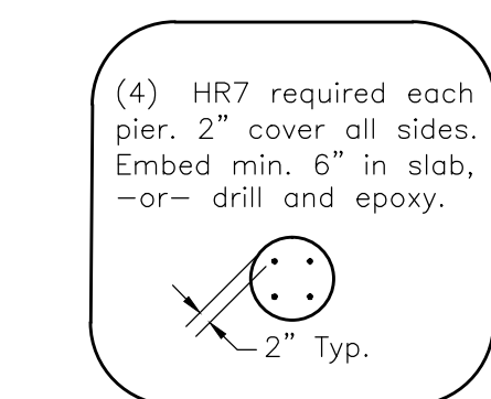
SAFETY PIER REINFORCING Top View
