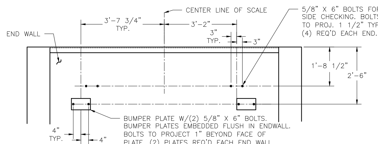
END WALL CHECKING DETAIL
